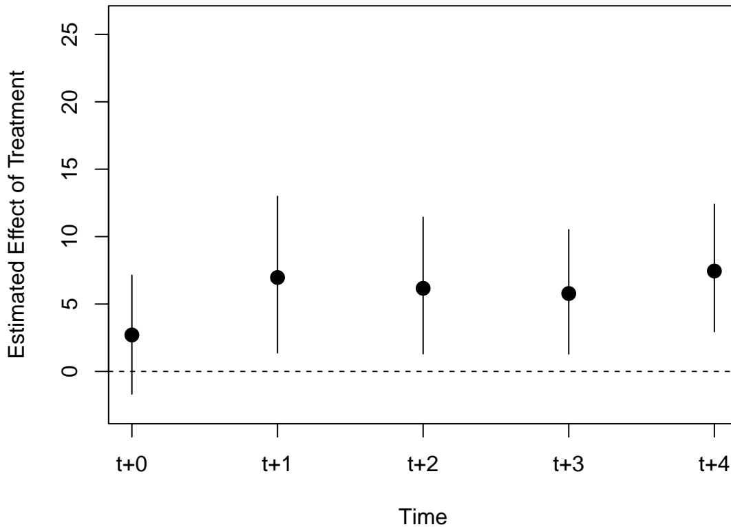
Figure J-10: PaneMatch
