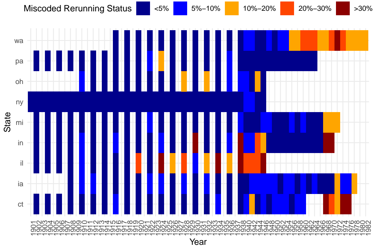
Figure 2: Mis-coded Rerunners
