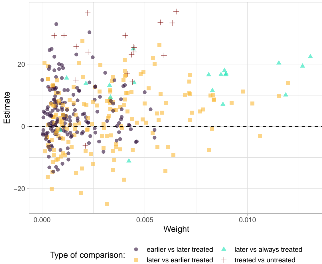
Figure G-4: Goodman-Bacon weights in two-way fixed effects estimation (post-1946)
