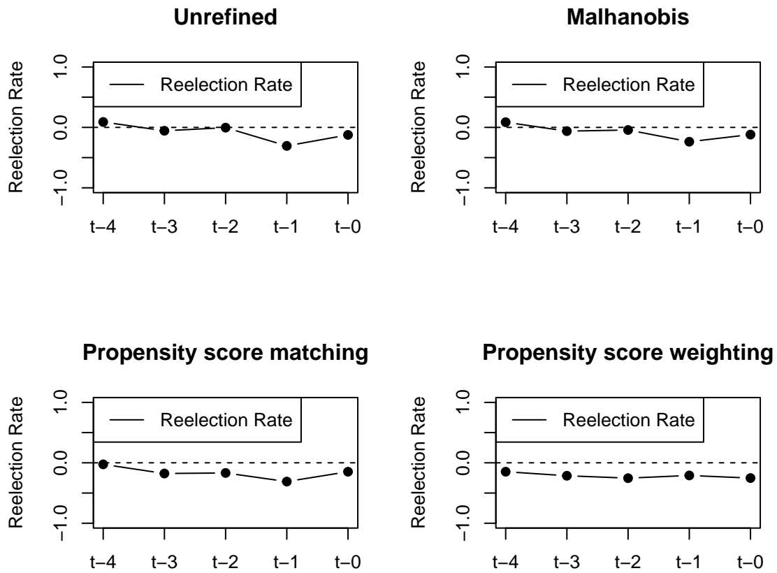
Figure J-8: Covariate
