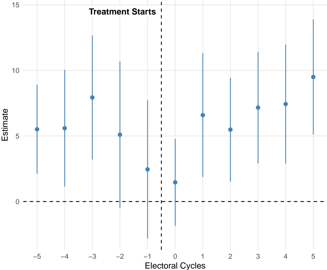
Figure 4: Treatment effects over time using imputation
