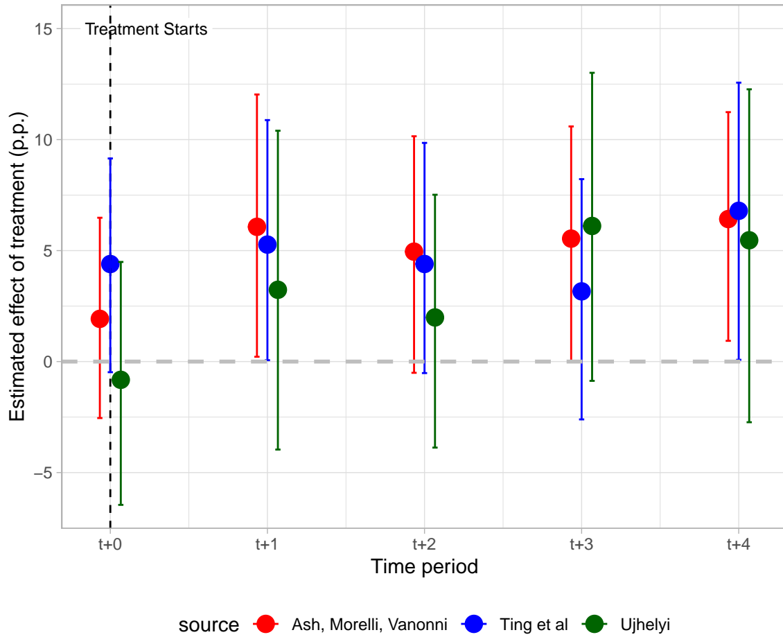
Figure F-3: Mahalanobis PanelMatch estimates: Comparison for the three sources for reform dates – Ash
