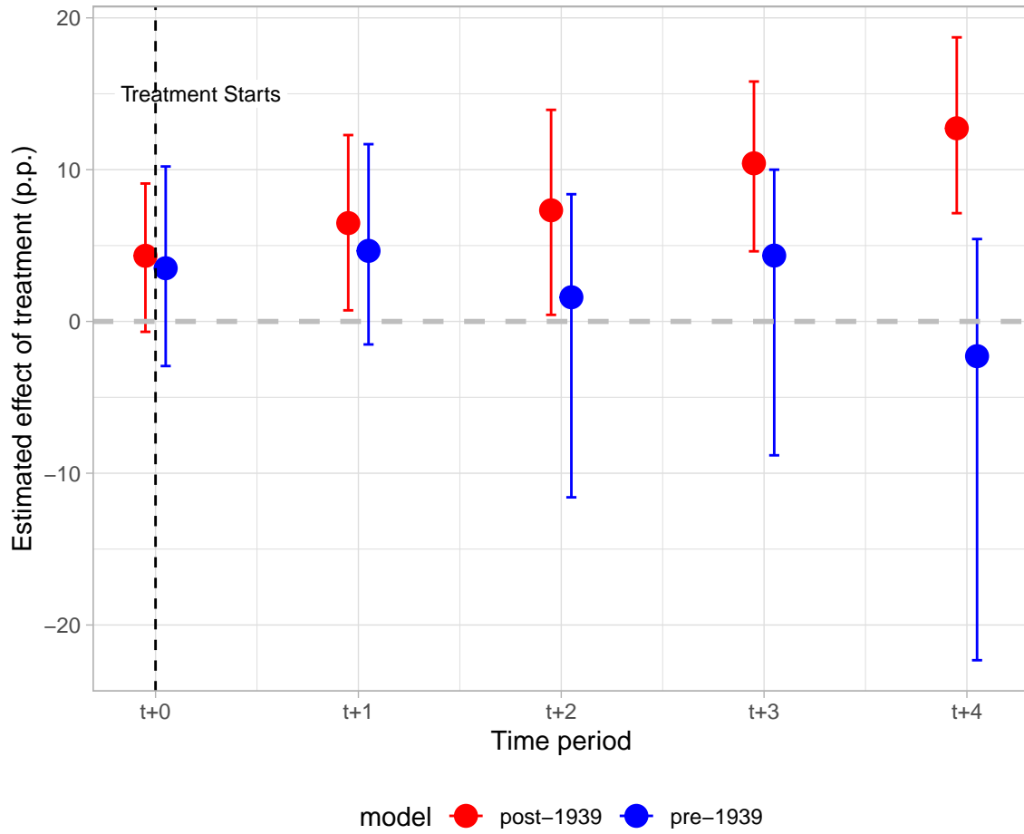
Figure J-11: PaneMatch for the subset of state-cycles before and after 1939
