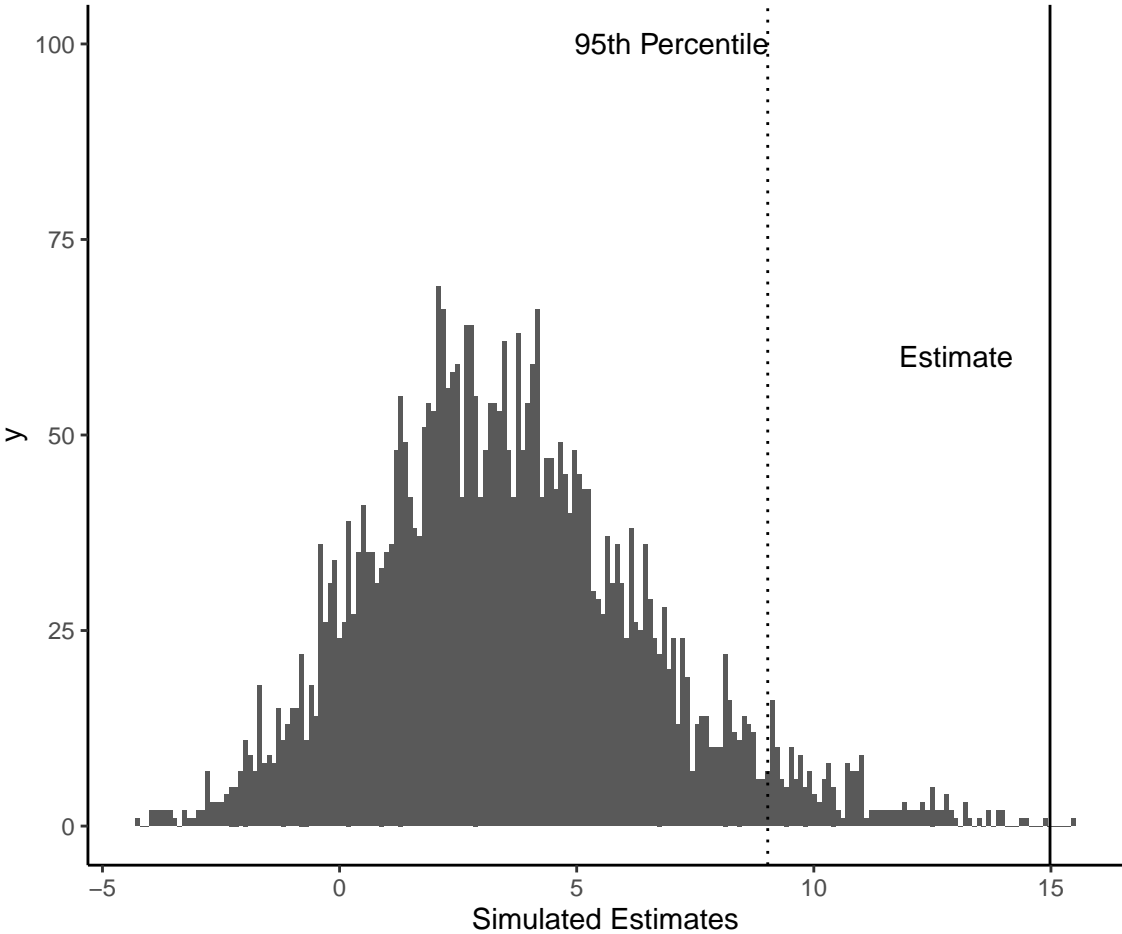
Figure I-5: Randomization inference with placebo treatments: using simulated treatment timings
