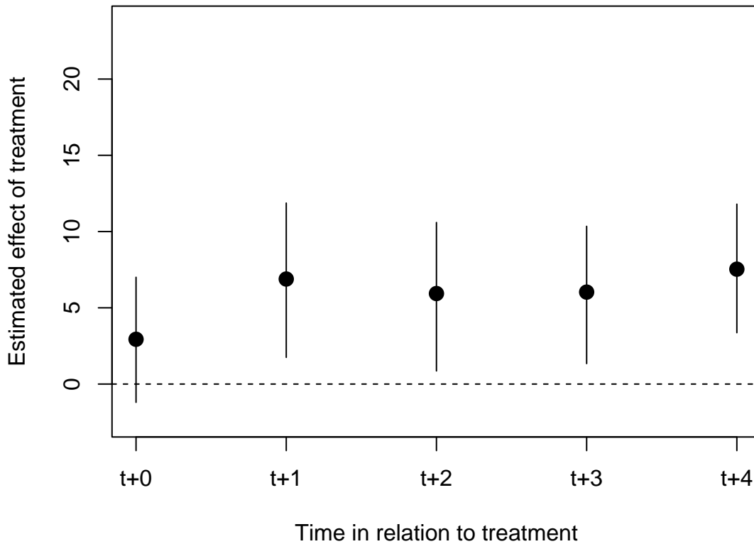
Figure J-7: Unrefined PanelMatch coefficient estimates
