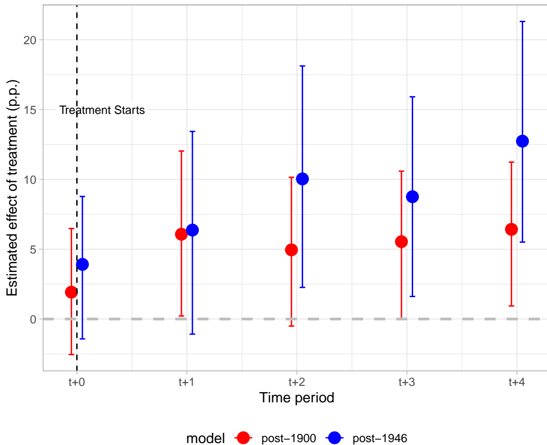
Figure E-2: Mahalanobis PanelMatch estimates for the full data (post-1900) and for the data post-1946
