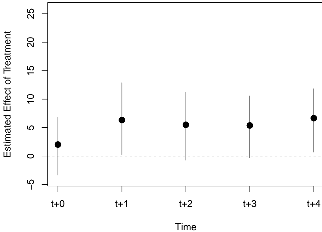
Figure J-9: PanelMatch
